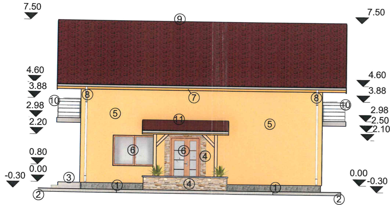
FATADA PRINCIPALA
